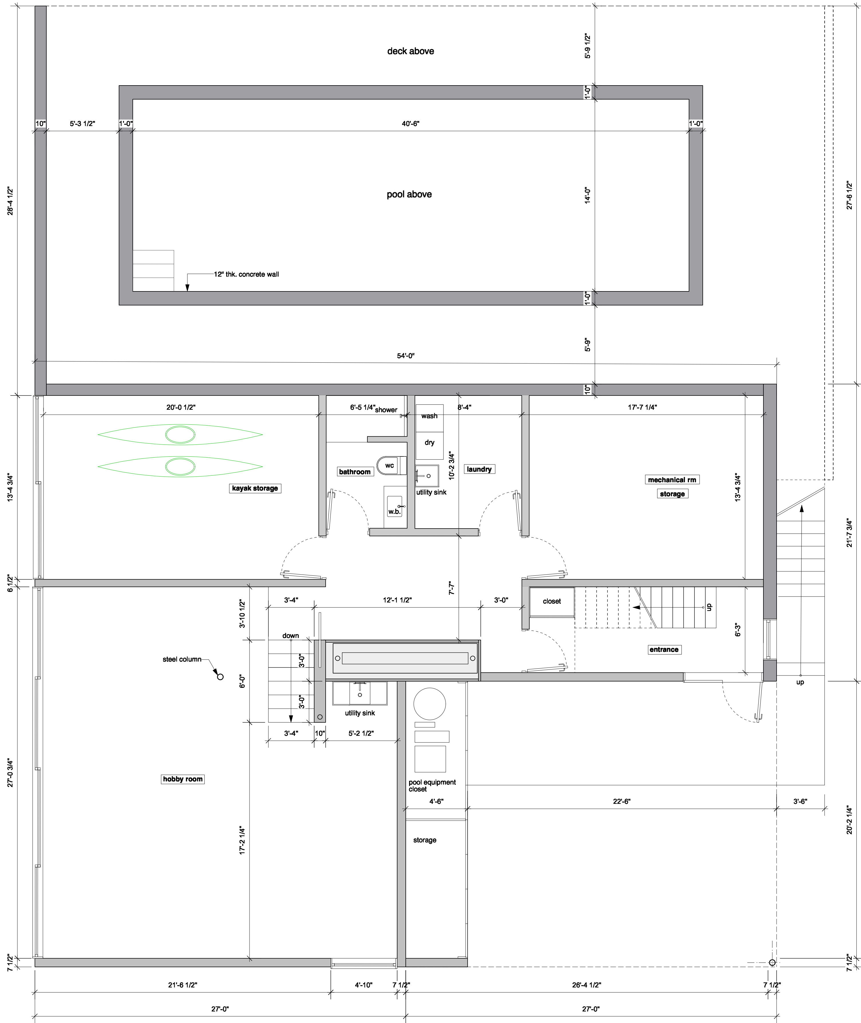
1 basement floor plan 1/4" = 1'
