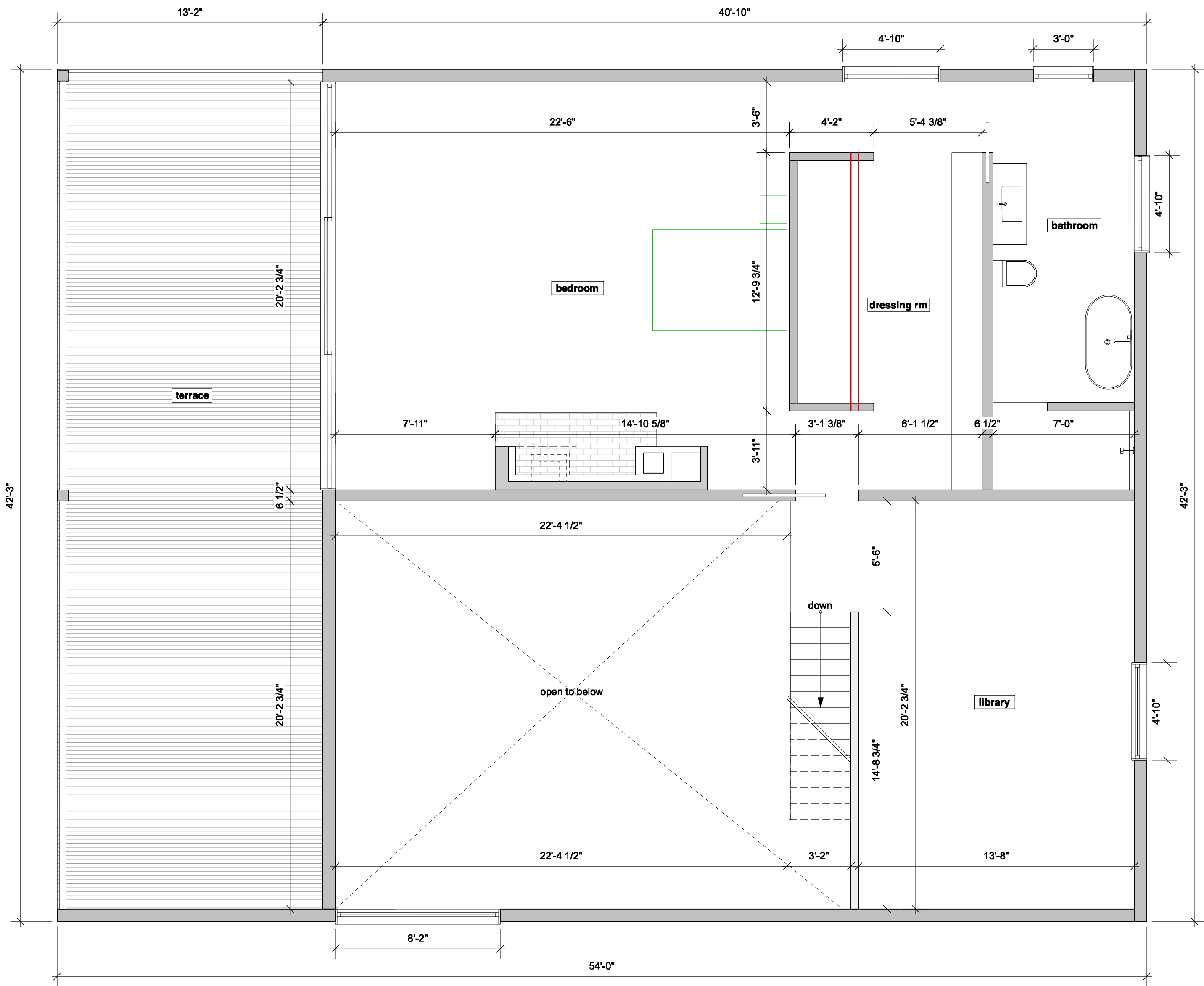
1 2nd floor plan 1/4" = 1'
