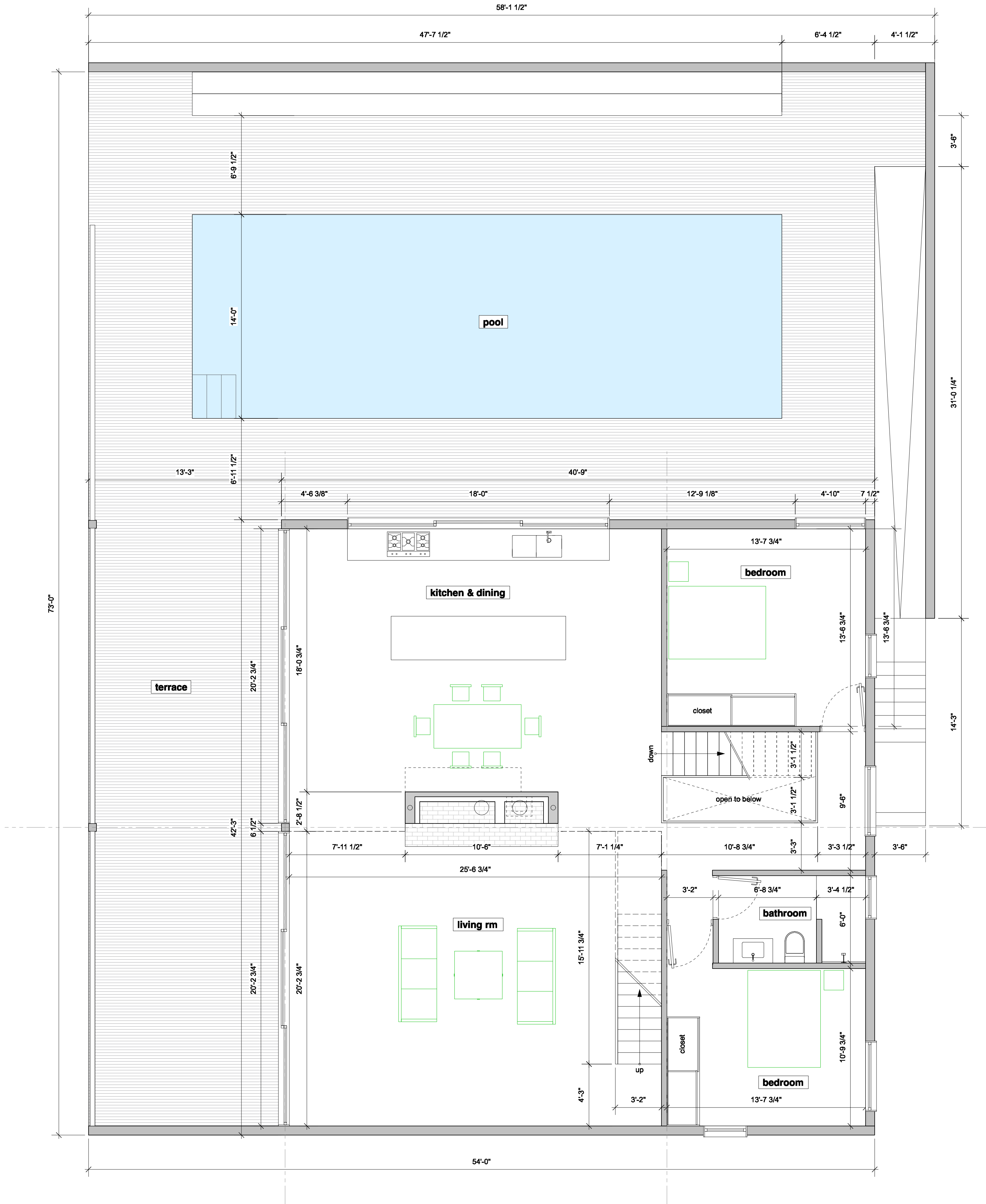
1 1st floor plan 1/4" = 1'
