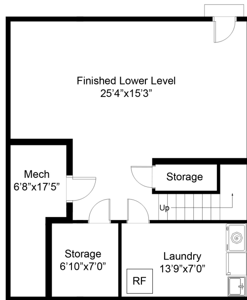
LOWER FLOOR PLAN
