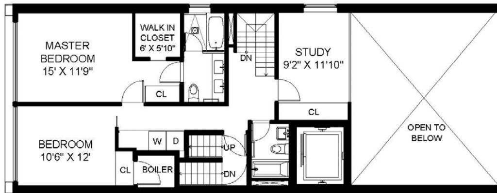
2nd FLOOR
