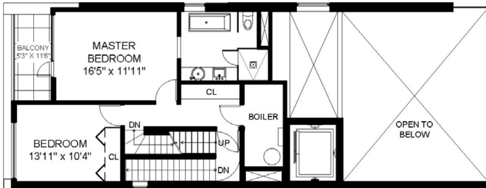
6th FLOOR
