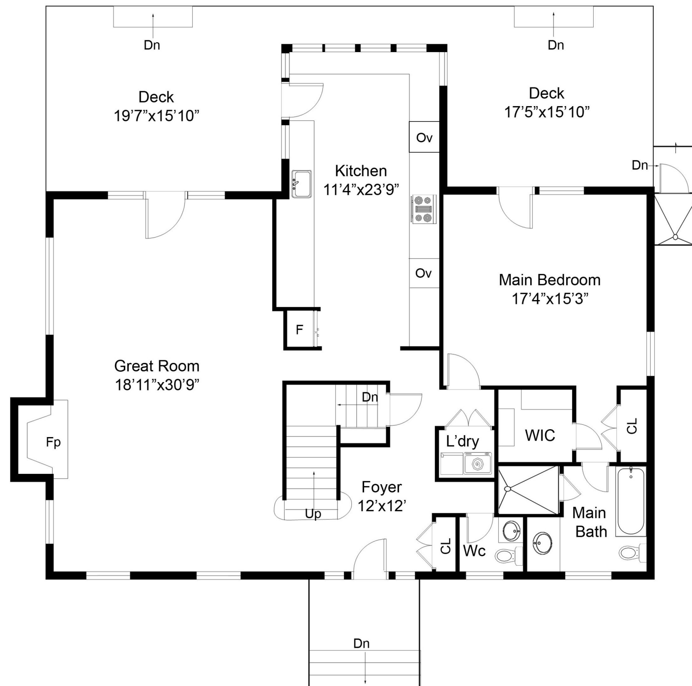
FLOOR PLAN
