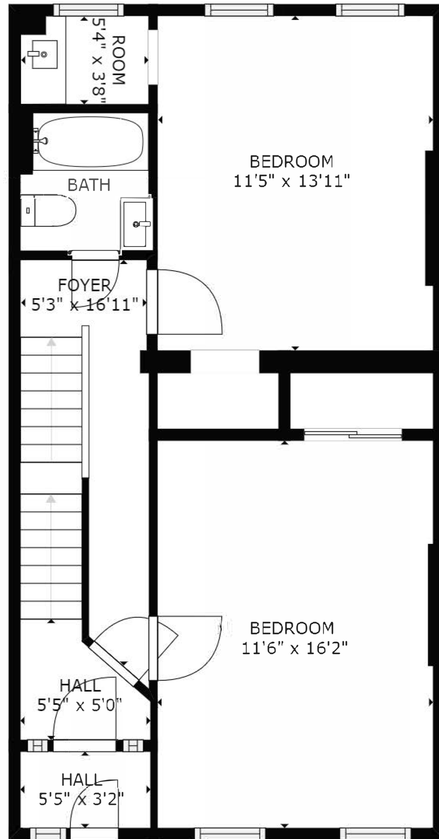
FLOOR 2
