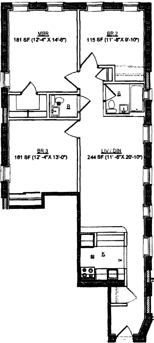
APT 'B,D,F,H,J' 3RD/5TH FLOOR UPPER LEVEL
