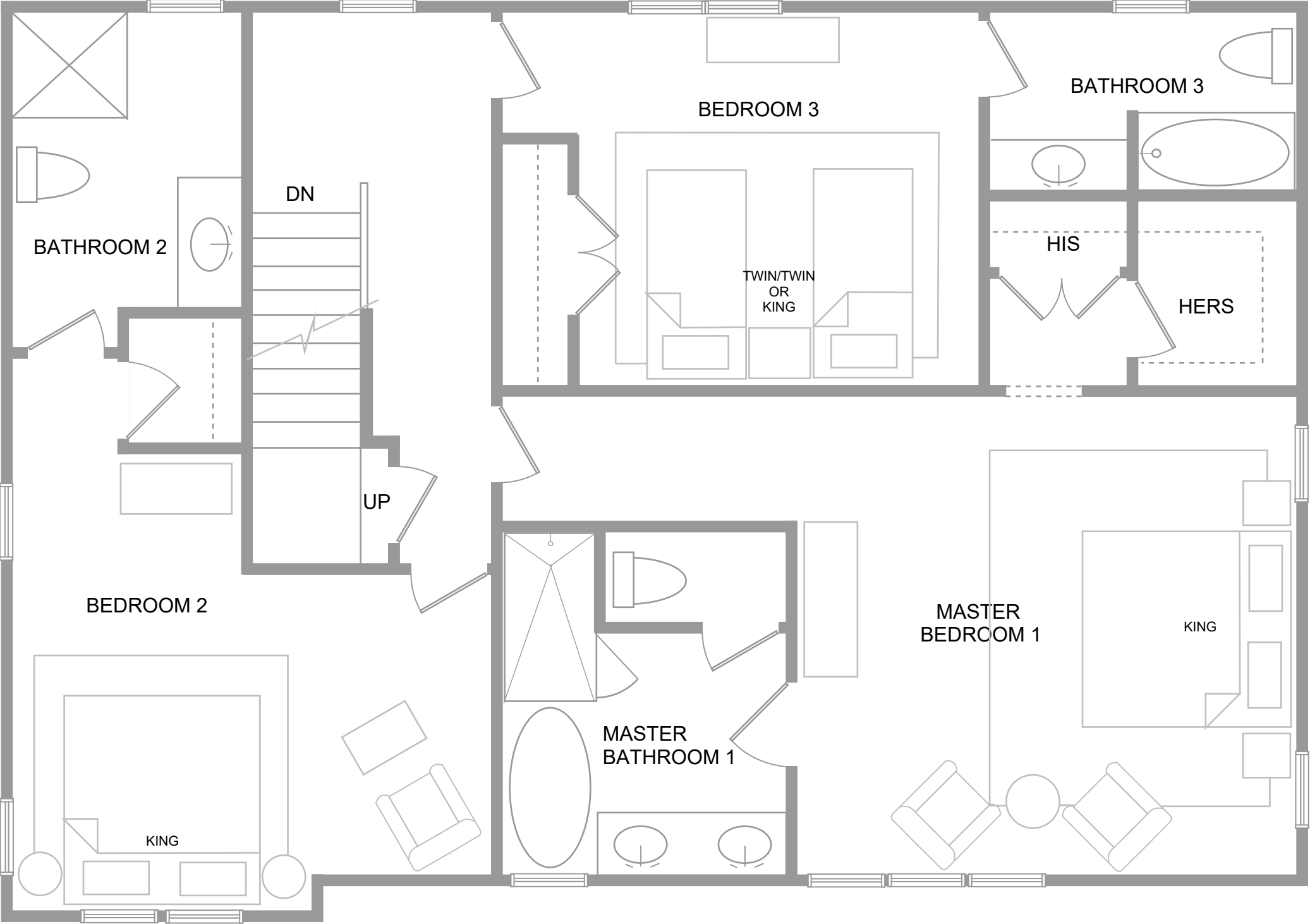
SECOND FLOOR
