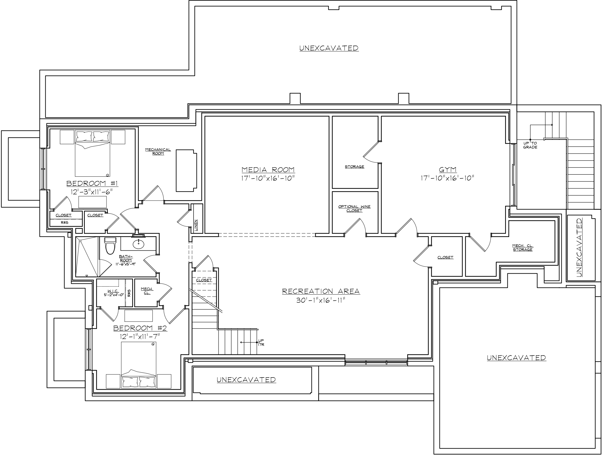
B A S E M E N T P L A N ( 1 2 - 1 9 - 1 7 ) T O W N L I N E R O A D L O T 1 4 1,989 SQ. FT.
