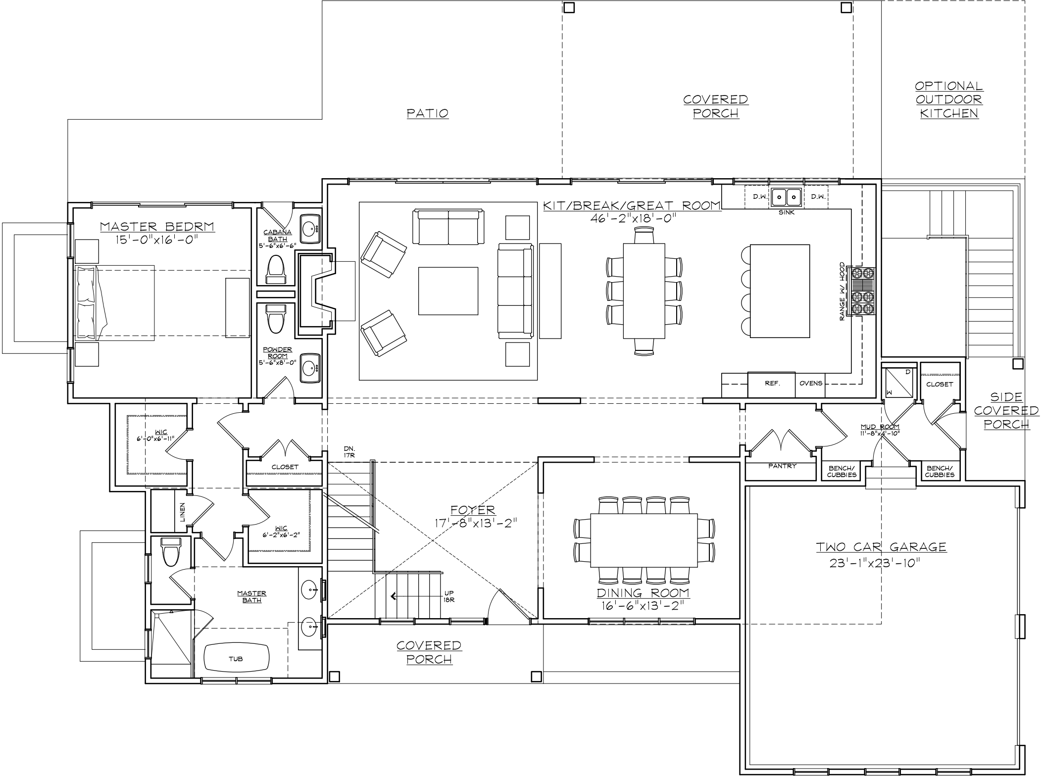
FIRST FLOOR PLAN (12-19-17) TOWN LINE ROAD LOT 14
