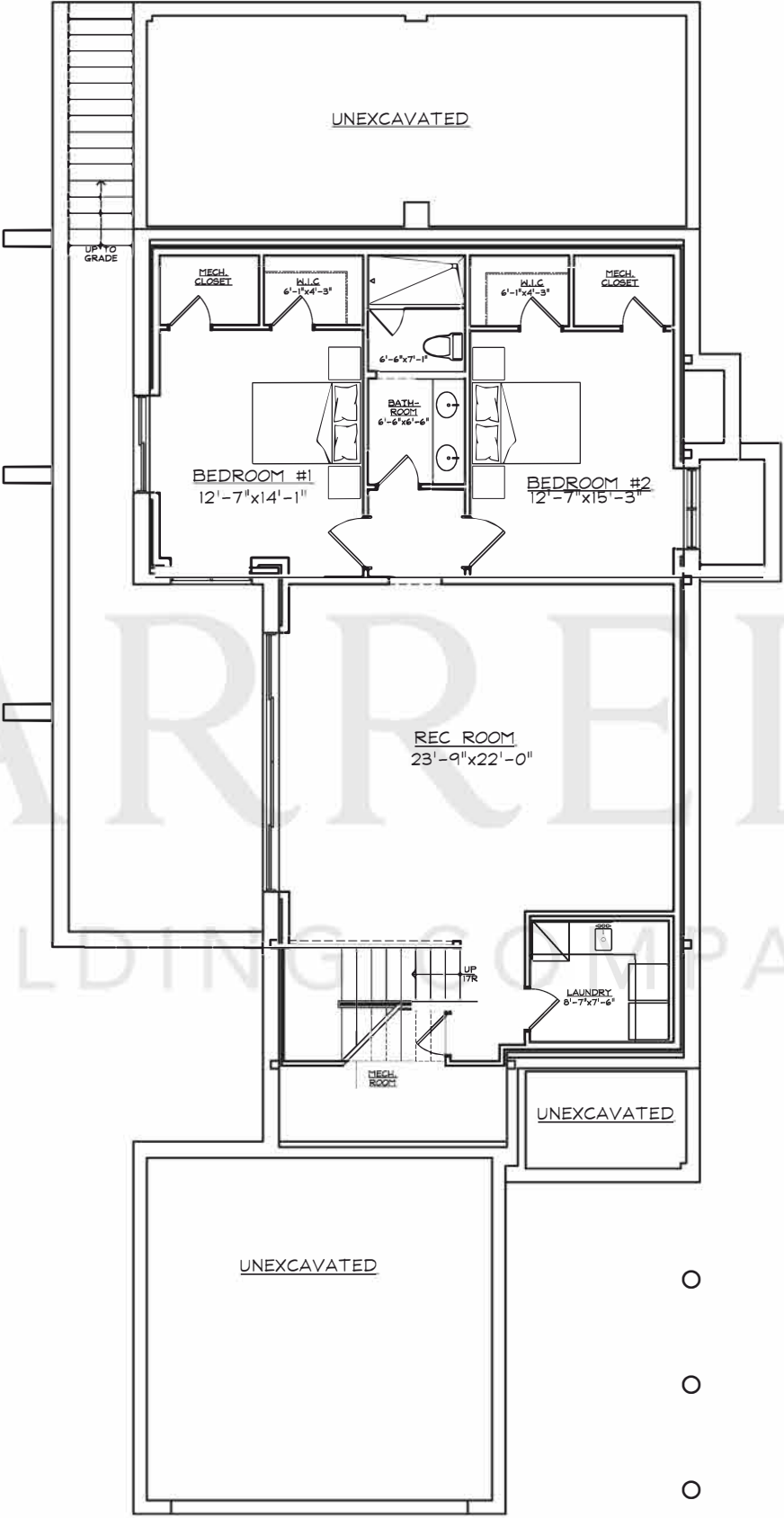
LOWER LEVEL PLAN (09-25-13) 54 MIANKOMA LANE 1,374 SF.
