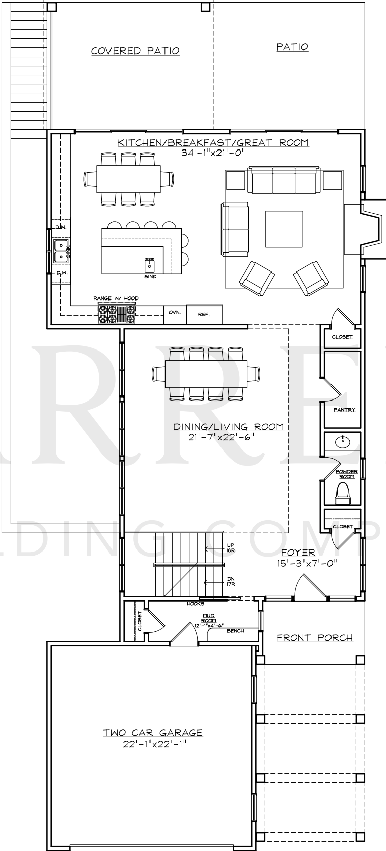
FIRST FLOOR PLAN (09-25-17) 54 MIANKOMA LANE 1,653 SQ.FT. TOTAL 2,885 SQ.FT.
