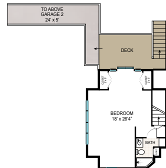
SECOND FLOOR OVER GARAGE 1
